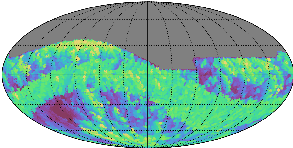
too_elab_r16_d2_griz_v3.4_10yrs All sky r band: Max airmass
