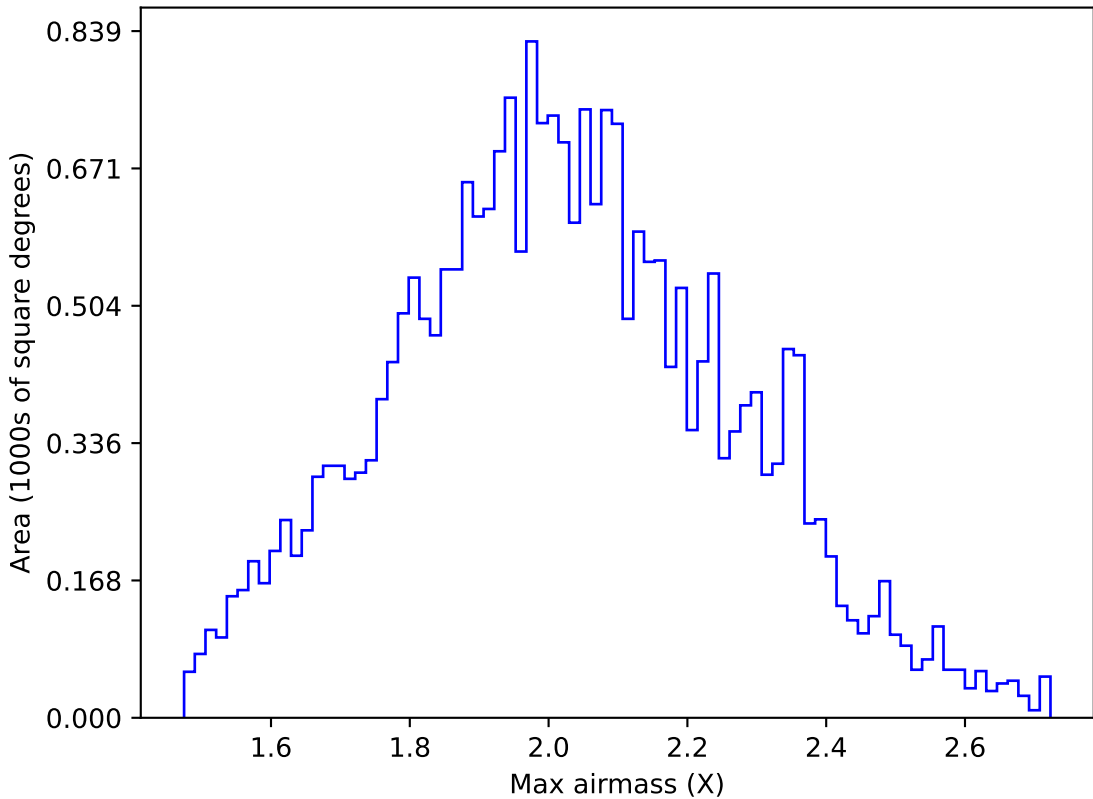
too_elab_r16_d2_griz_v3.4_10yrs All sky g band: Max airmass
