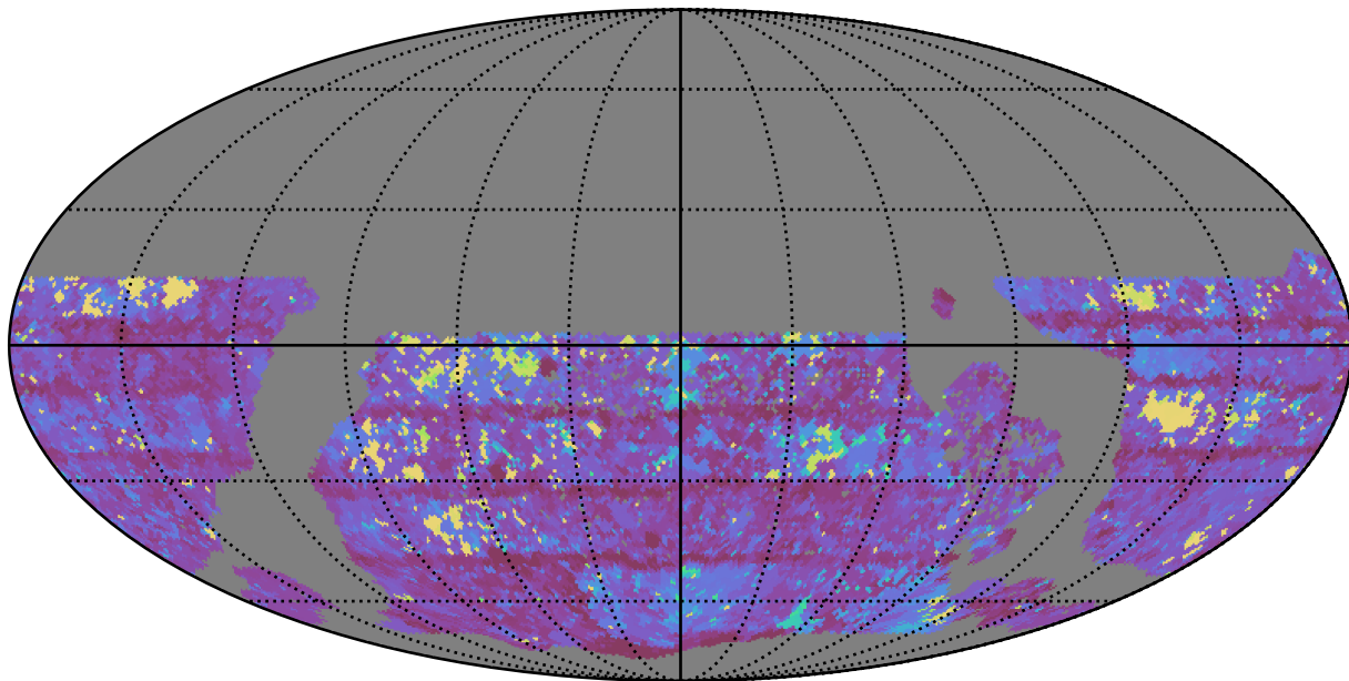
too_elab_r16_d2_griz_v3.4_10yrs WFD y band: Max Inter-Night Gap
