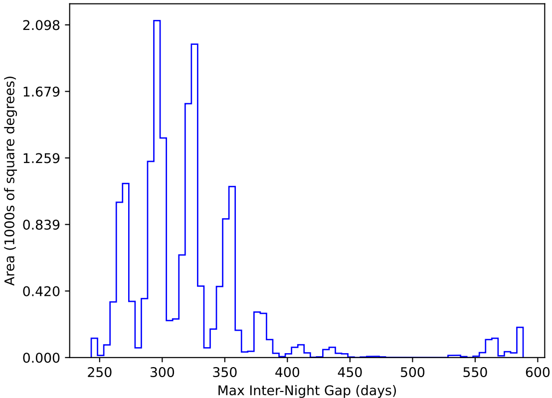
too_elab_r16_d2_griz_v3.4_10yrs WFD y band: Max Inter-Night Gap
