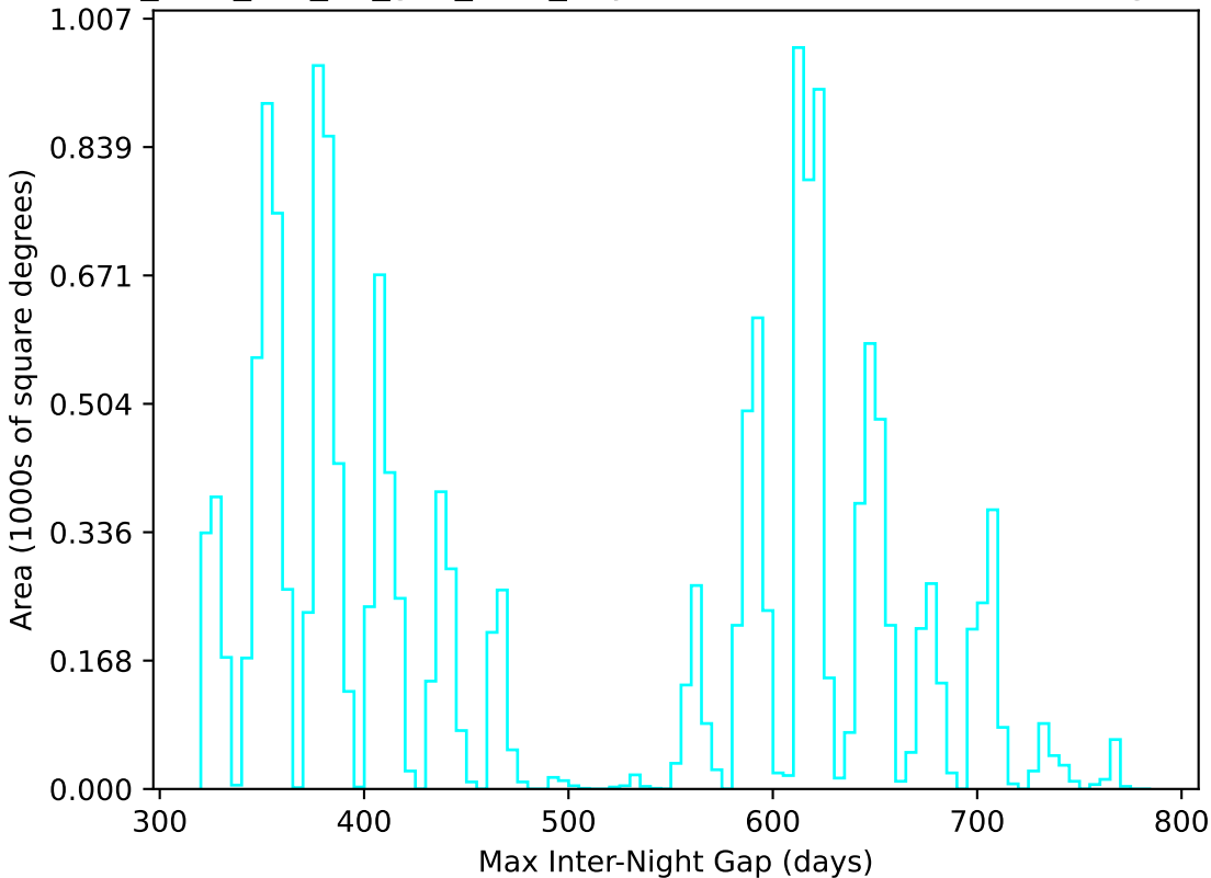
too_elab_r16_d2_griz_v3.4_10yrs WFD u band: Max Inter-Night Gap
