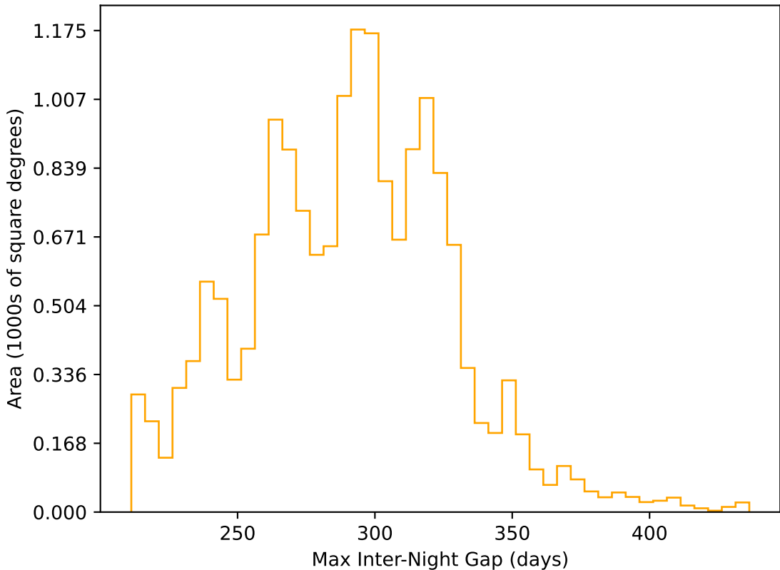
too_elab_r16_d2_griz_v3.4_10yrs WFD r band: Max Inter-Night Gap
