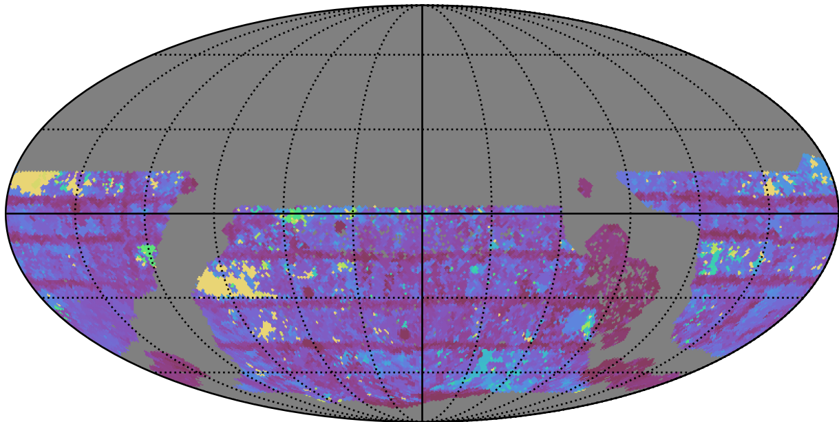
too_elab_r16_d2_griz_v3.4_10yrs WFD i band: Max Inter-Night Gap
