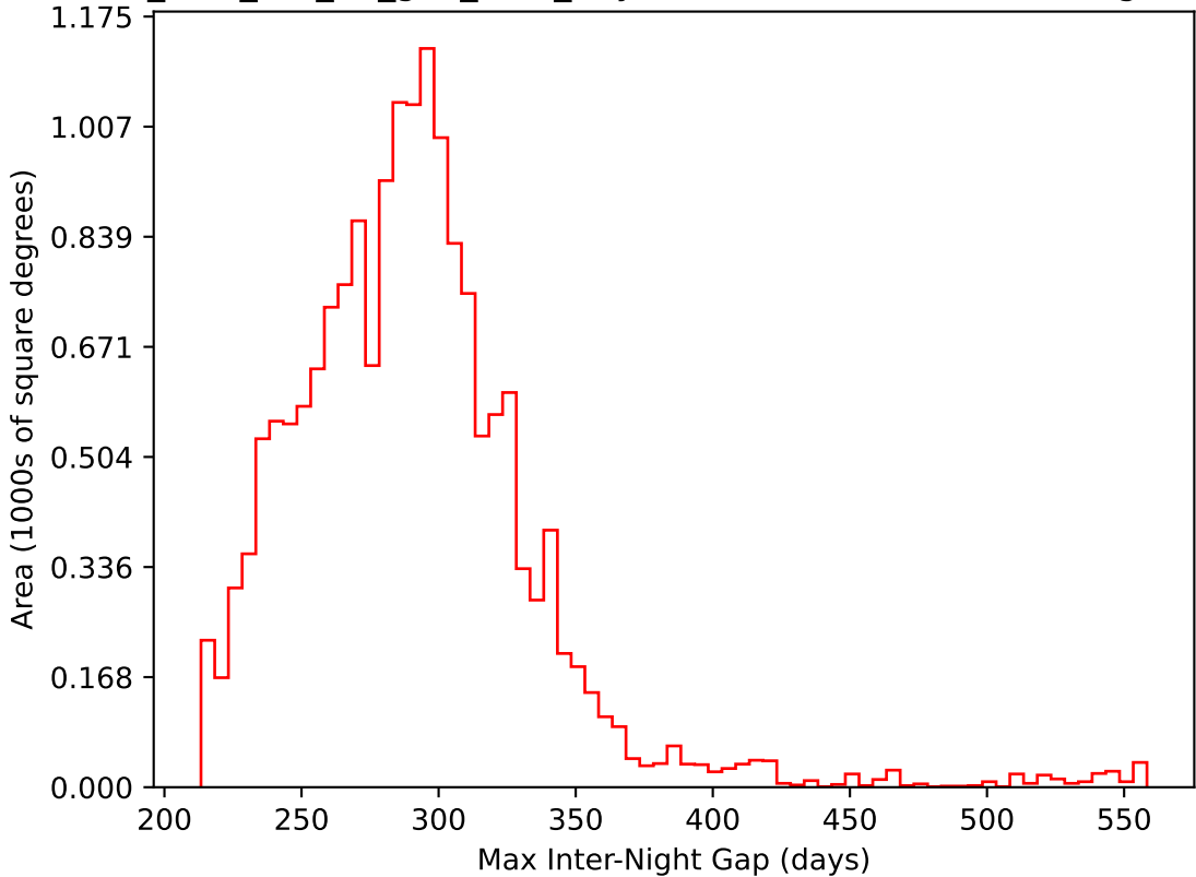
too_elab_r16_d2_griz_v3.4_10yrs WFD i band: Max Inter-Night Gap
