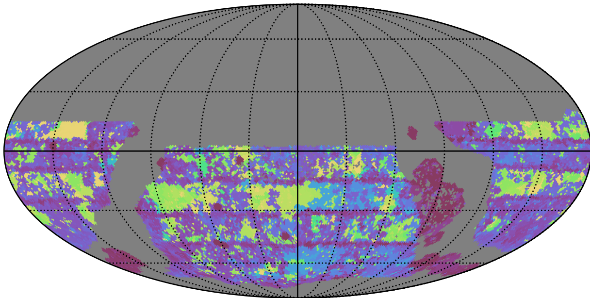
too_elab_r16_d2_griz_v3.4_10yrs WFD g band: Max Inter-Night Gap
