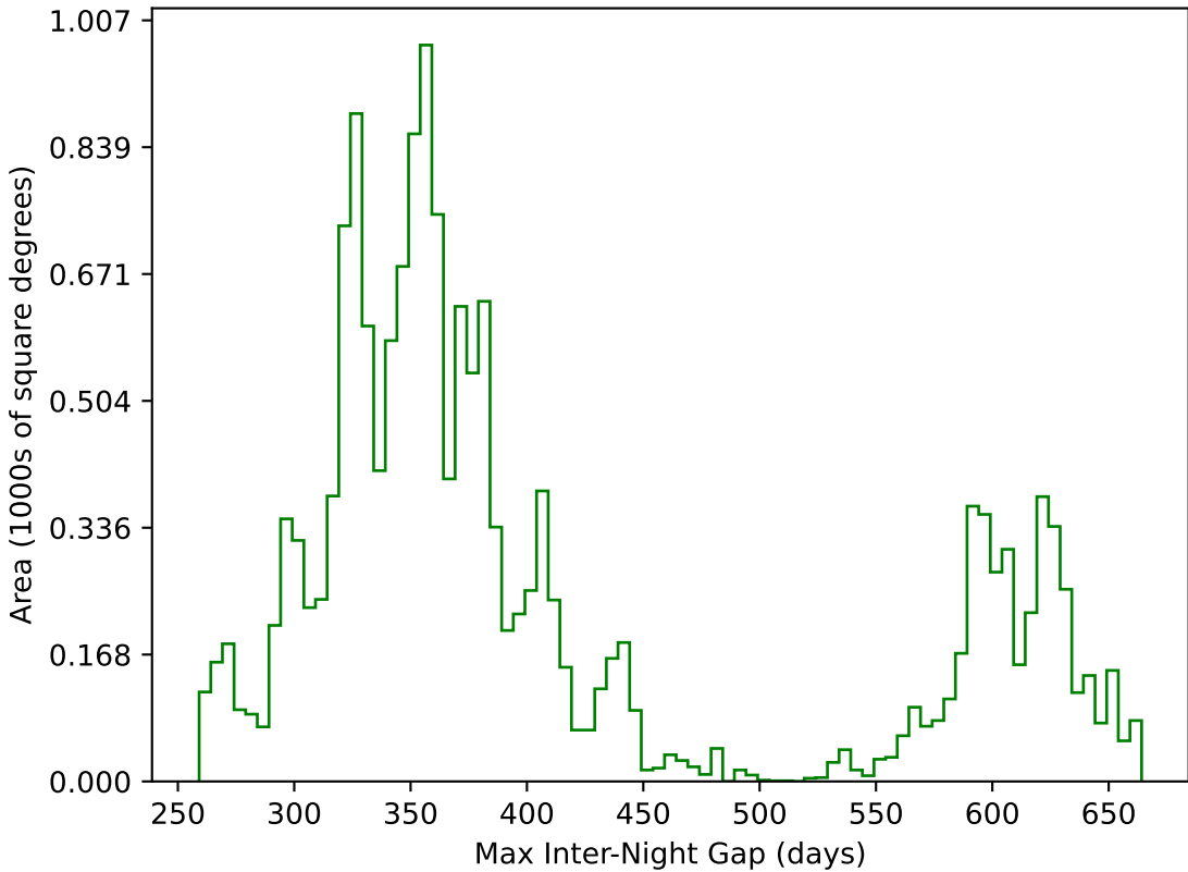
too_elab_r16_d2_griz_v3.4_10yrs WFD g band: Max Inter-Night Gap
