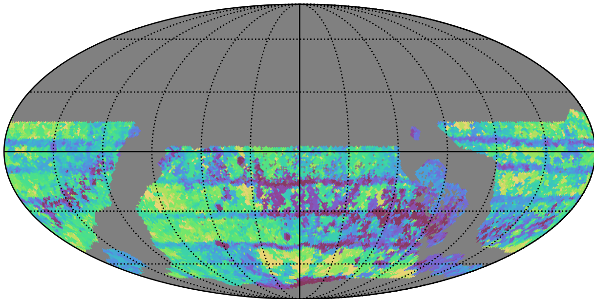
too_elab_r16_d2_griz_v3.4_10yrs WFD all bands: Max Inter-Night Gap
