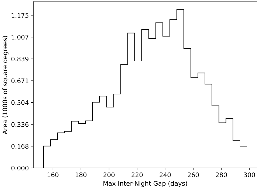
too_elab_r16_d2_griz_v3.4_10yrs WFD all bands: Max Inter-Night Gap
