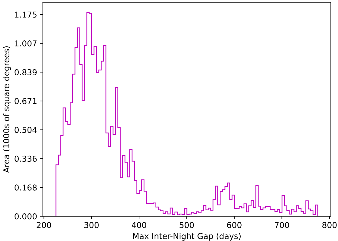
too_elab_r16_d2_griz_v3.4_10yrs All sky z band: Max Inter-Night Gap
