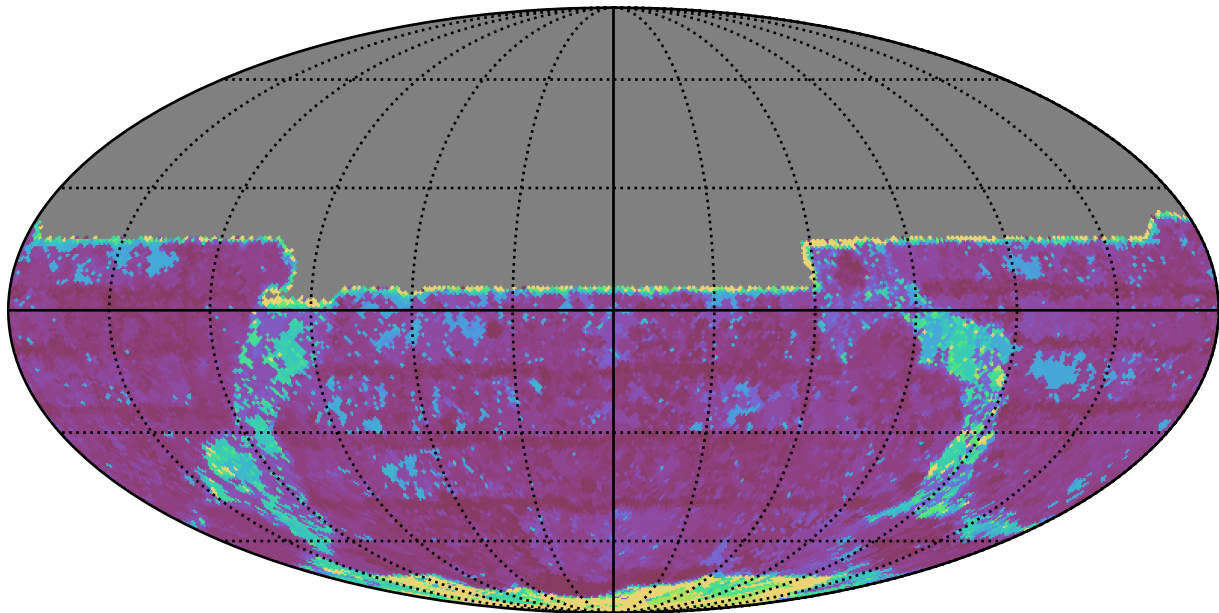
too_elab_r16_d2_griz_v3.4_10yrs All sky y band: Max Inter-Night Gap
