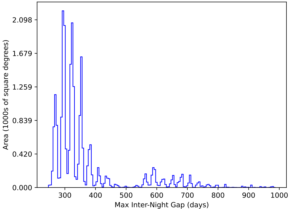
too_elab_r16_d2_griz_v3.4_10yrs All sky y band: Max Inter-Night Gap
