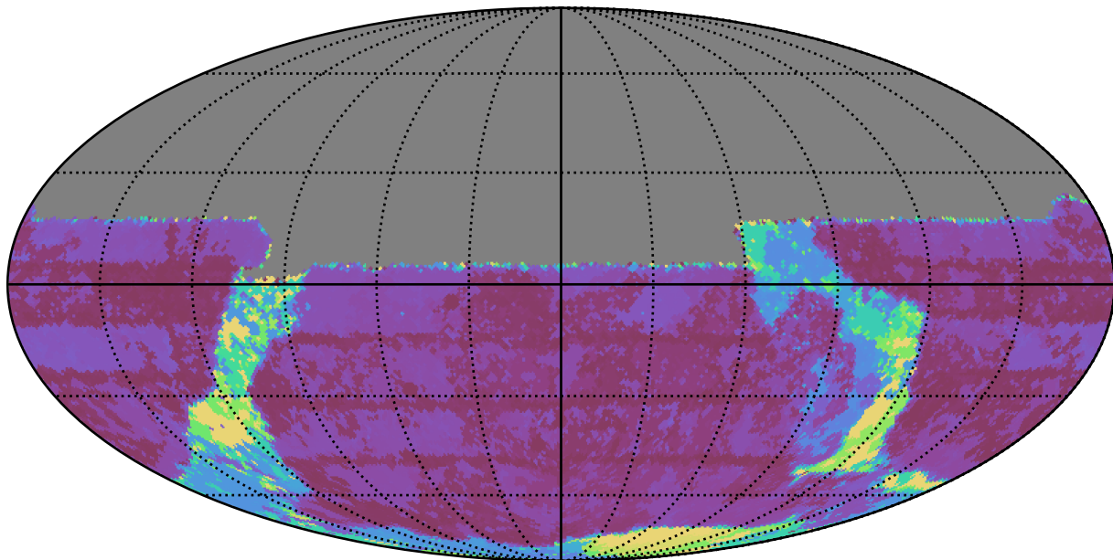
too_elab_r16_d2_griz_v3.4_10yrs All sky u band: Max Inter-Night Gap
