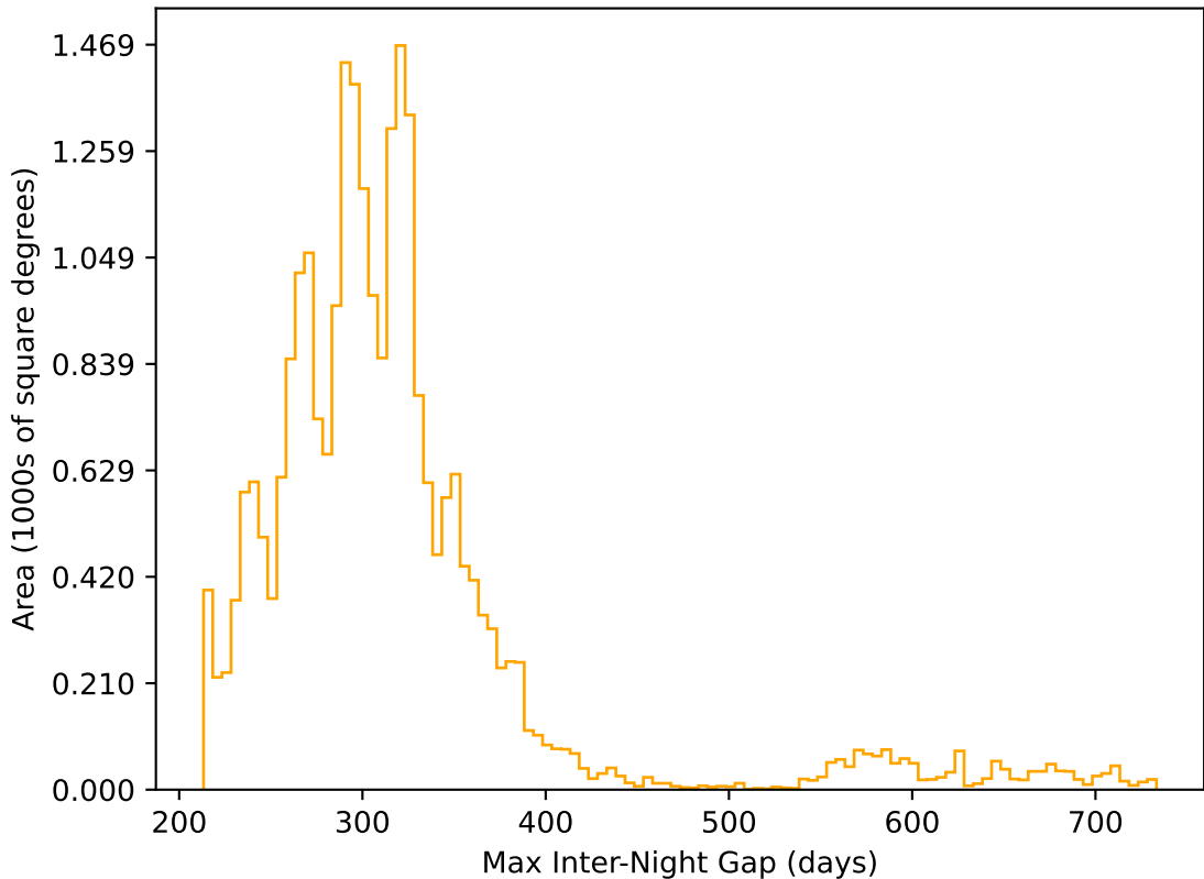
too_elab_r16_d2_griz_v3.4_10yrs All sky r band: Max Inter-Night Gap
