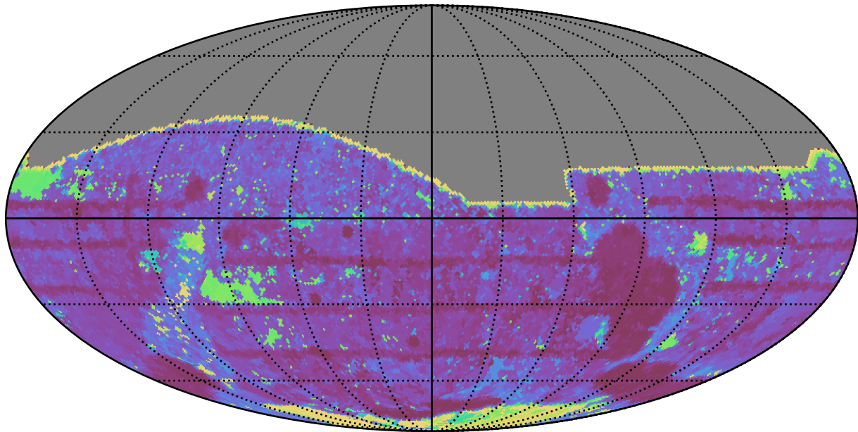
too_elab_r16_d2_griz_v3.4_10yrs All sky i band: Max Inter-Night Gap
