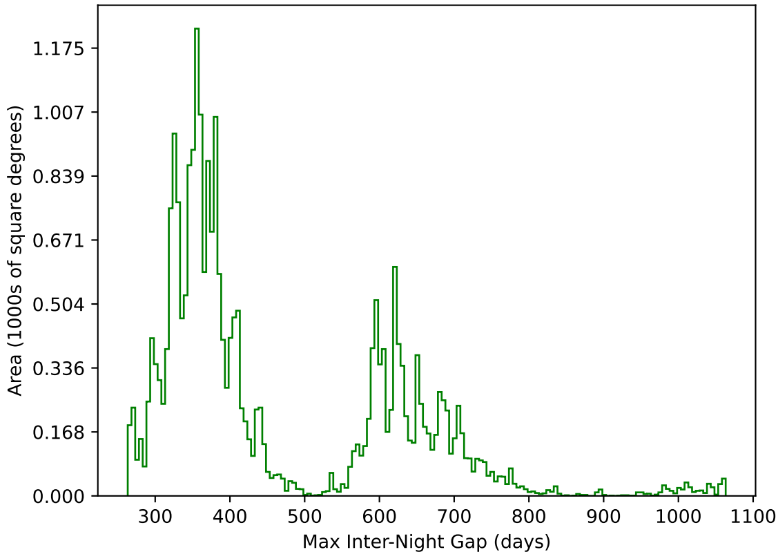
too_elab_r16_d2_griz_v3.4_10yrs All sky g band: Max Inter-Night Gap
