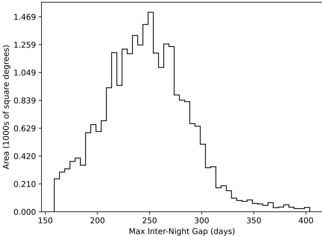
too_elab_r16_d2_griz_v3.4_10yrs All sky all bands: Max Inter-Night Gap
