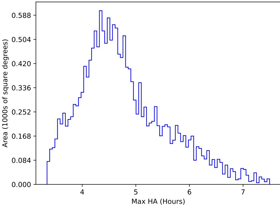
too_elab_r16_d2_griz_v3.4_10yrs WFD y band: Max HA
