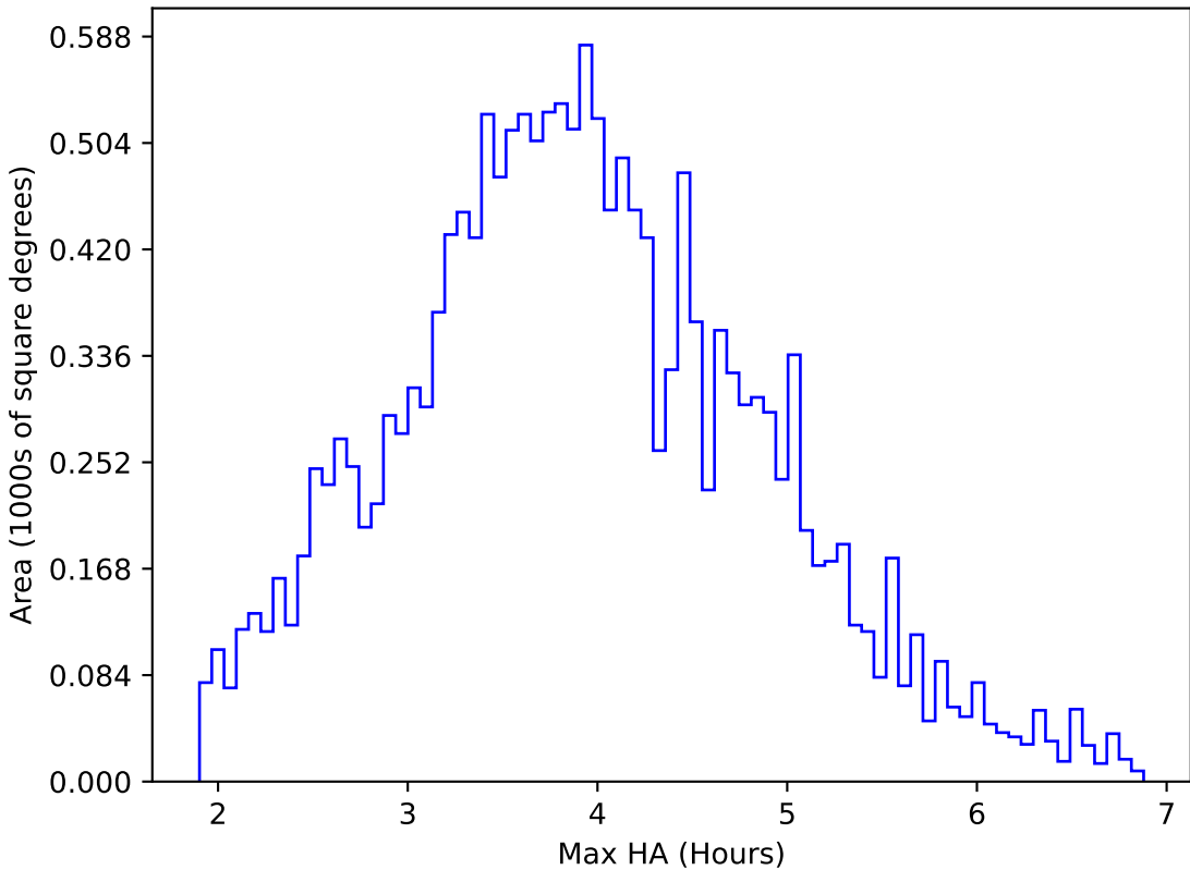
too_elab_r16_d2_griz_v3.4_10yrs WFD u band: Max HA
