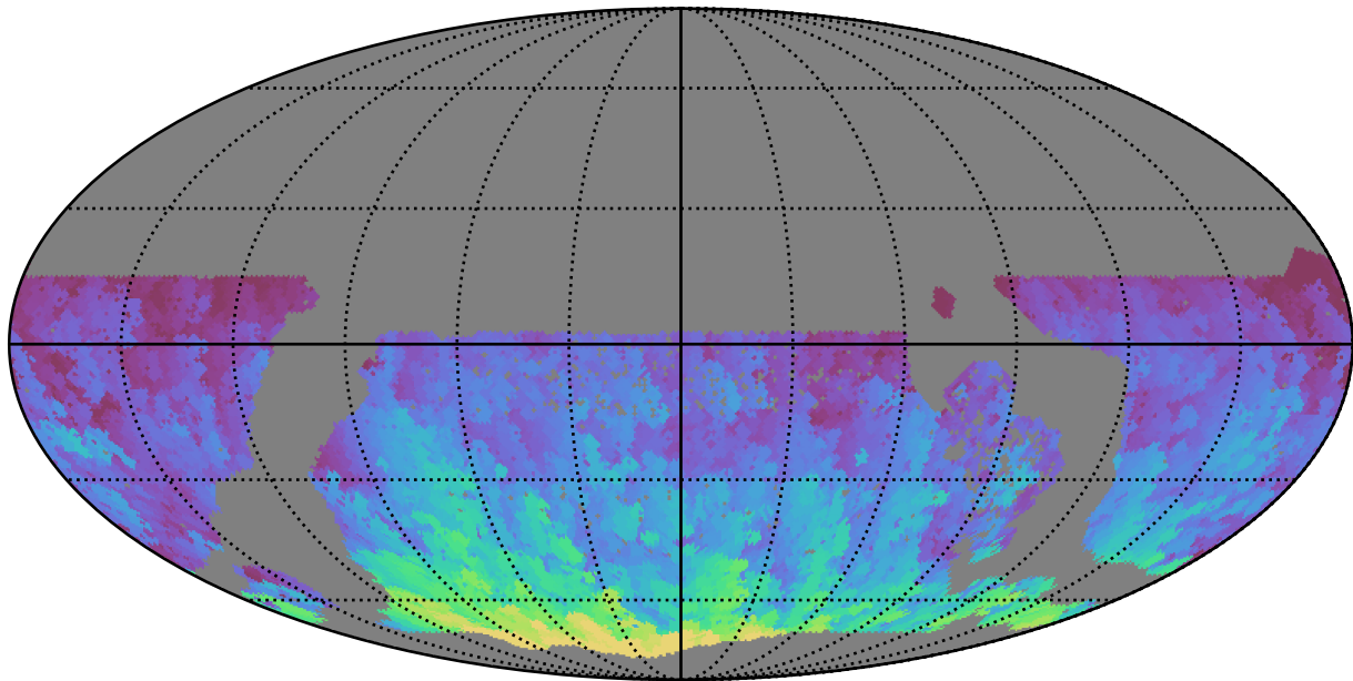
too_elab_r16_d2_griz_v3.4_10yrs WFD r band: Max HA
