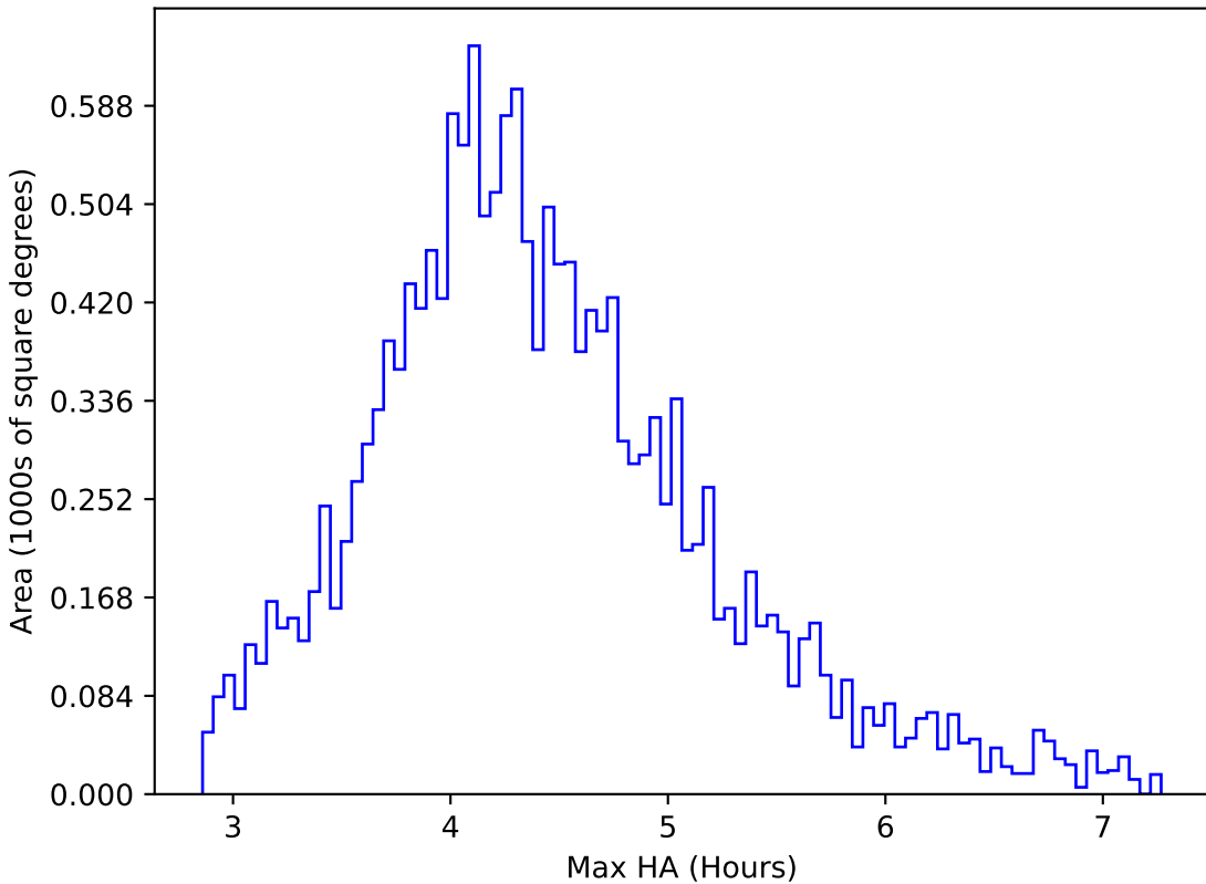
too_elab_r16_d2_griz_v3.4_10yrs WFD r band: Max HA
