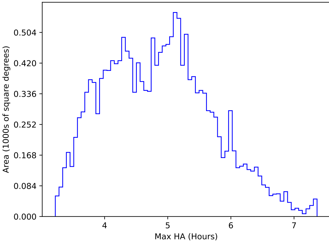
too_elab_r16_d2_griz_v3.4_10yrs WFD i band: Max HA
