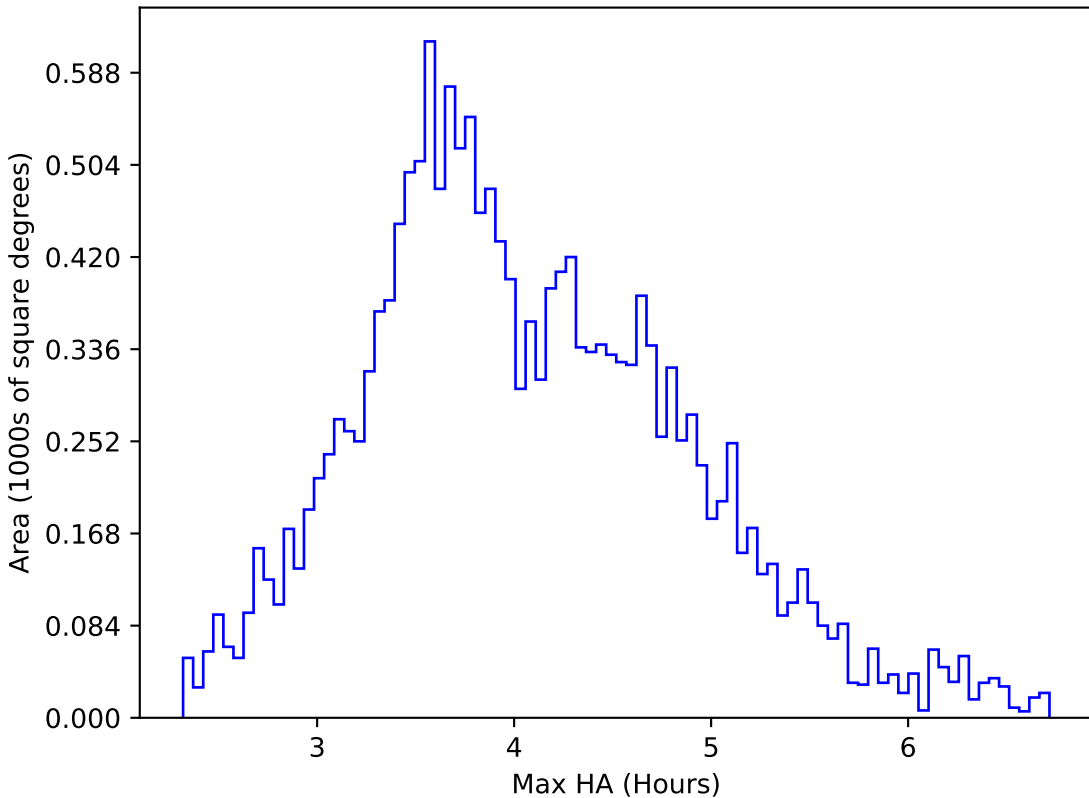
too_elab_r16_d2_griz_v3.4_10yrs WFD g band: Max HA
