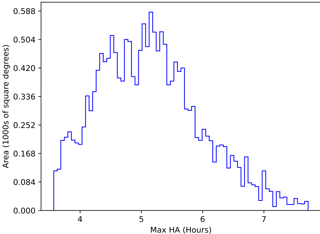
too_elab_r16_d2_griz_v3.4_10yrs WFD all bands: Max HA
