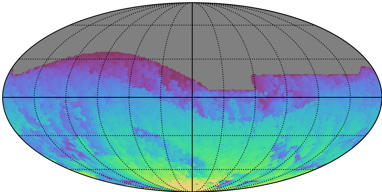
too_elab_r16_d2_griz_v3.4_10yrs All sky z band: Max HA
