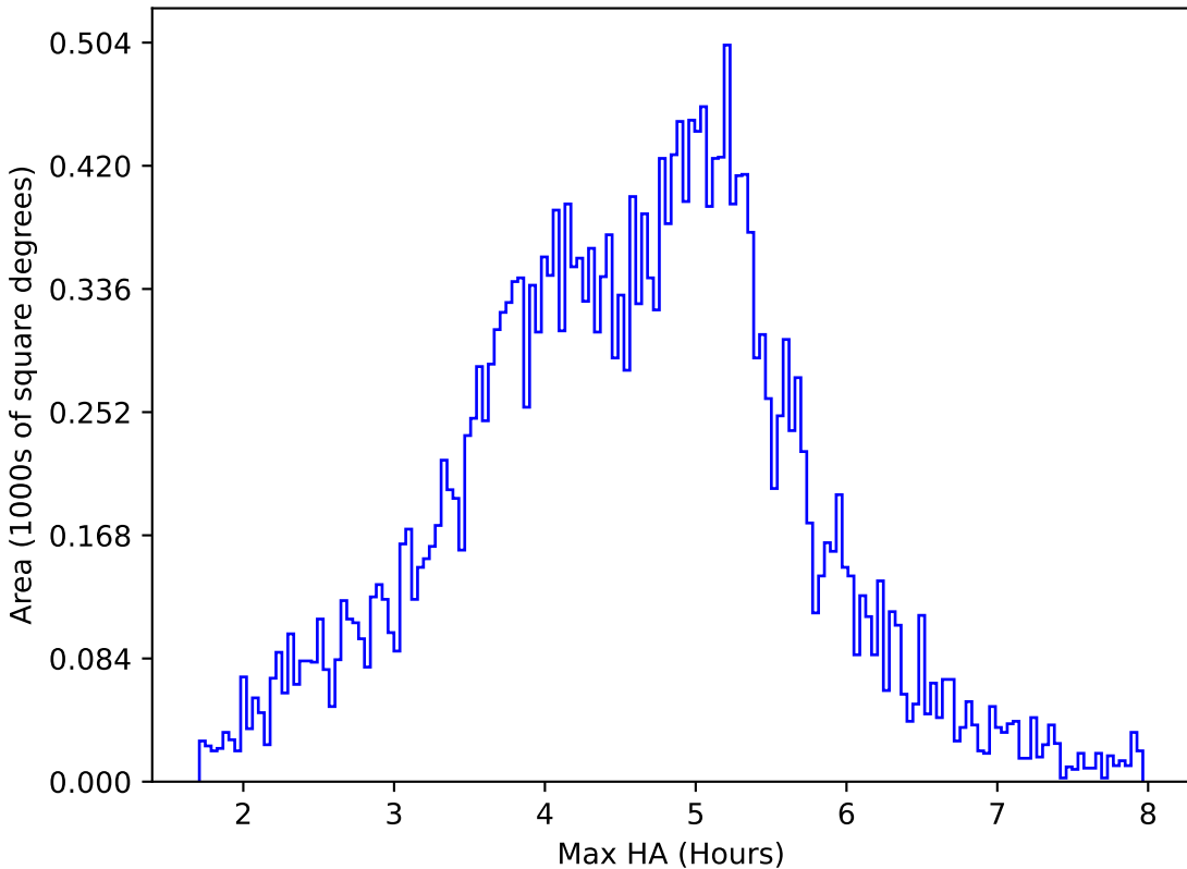
too_elab_r16_d2_griz_v3.4_10yrs All sky z band: Max HA
