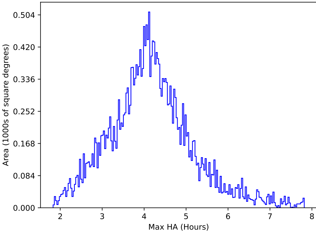
too_elab_r16_d2_griz_v3.4_10yrs All sky r band: Max HA
