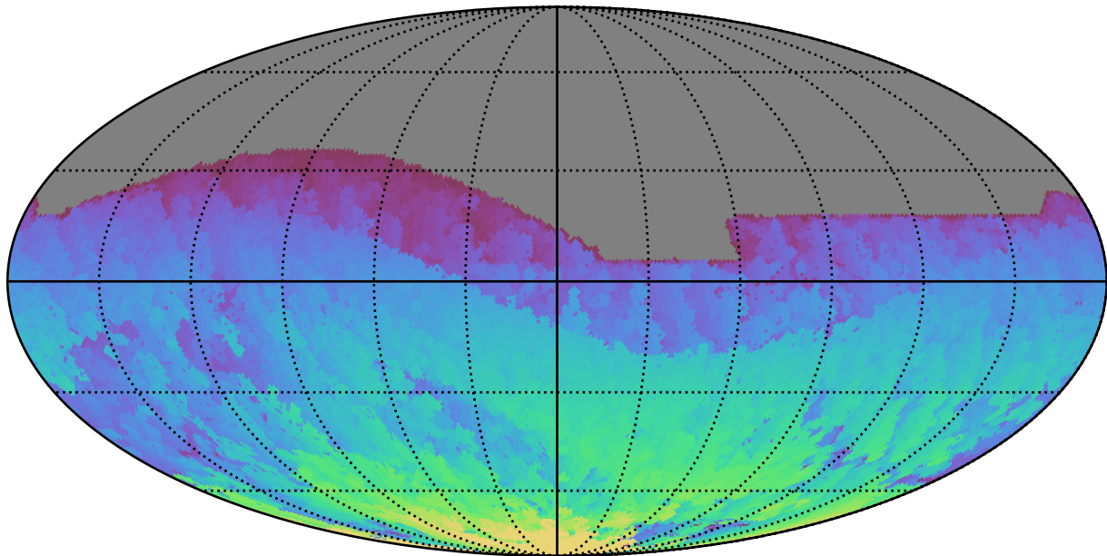
too_elab_r16_d2_griz_v3.4_10yrs All sky i band: Max HA
