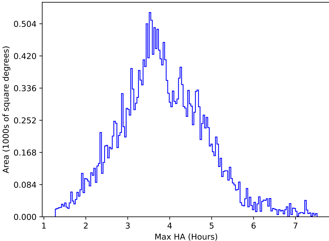
too_elab_r16_d2_griz_v3.4_10yrs All sky g band: Max HA
