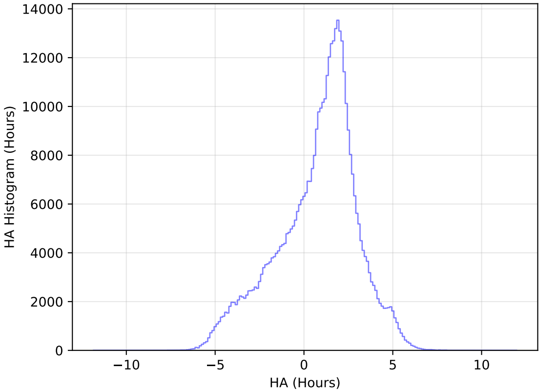
too_elab_r16_d2_griz_v3.4_10yrs WFD z band: HA Histogram
