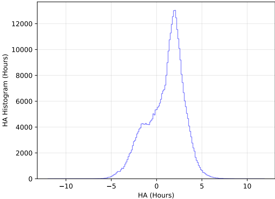
too_elab_r16_d2_griz_v3.4_10yrs WFD y band: HA Histogram
