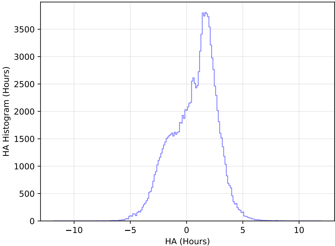
too_elab_r16_d2_griz_v3.4_10yrs WFD u band: HA Histogram
