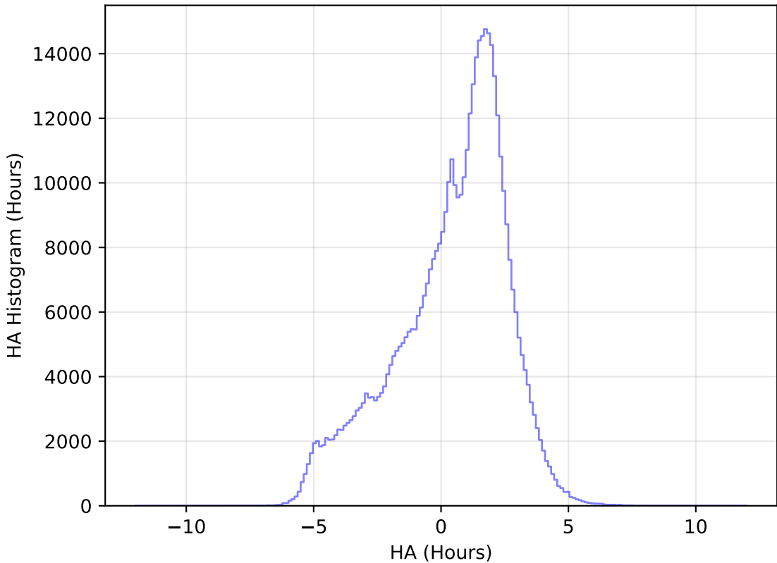
too_elab_r16_d2_griz_v3.4_10yrs WFD r band: HA Histogram
