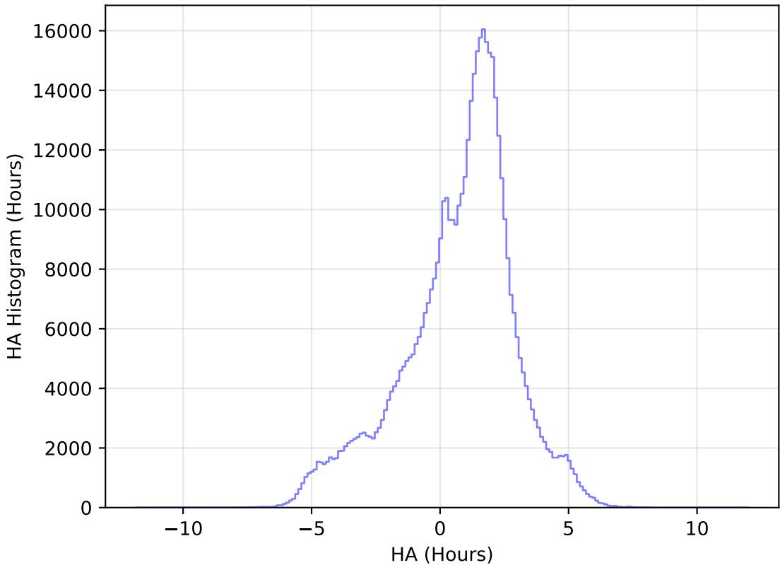
too_elab_r16_d2_griz_v3.4_10yrs WFD i band: HA Histogram
