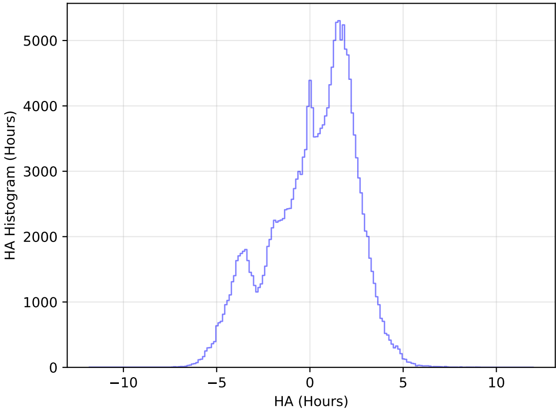
too_elab_r16_d2_griz_v3.4_10yrs WFD g band: HA Histogram
