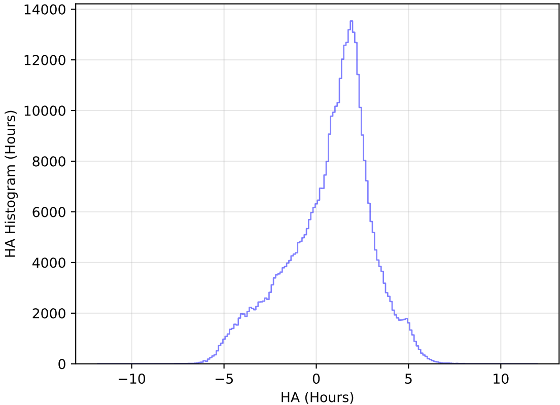
too_elab_r16_d2_griz_v3.4_10yrs All sky z band: HA Histogram
