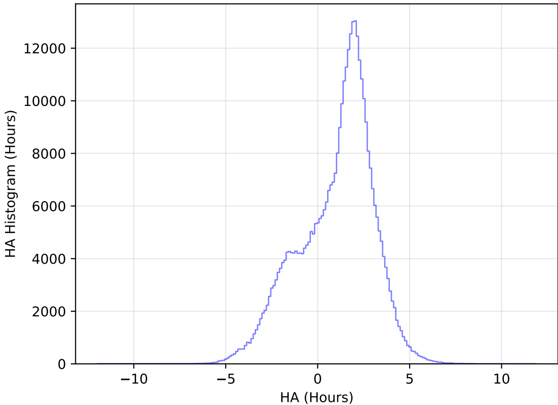
too_elab_r16_d2_griz_v3.4_10yrs All sky y band: HA Histogram
