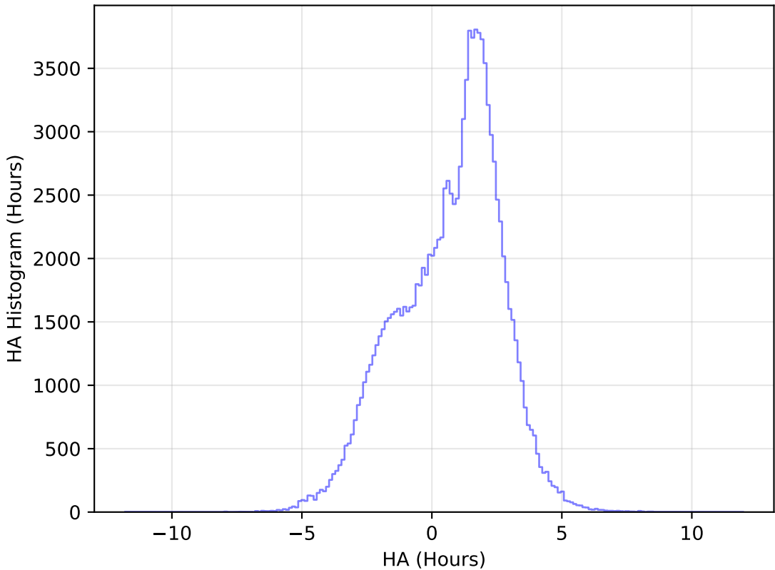
too_elab_r16_d2_griz_v3.4_10yrs All sky u band: HA Histogram
