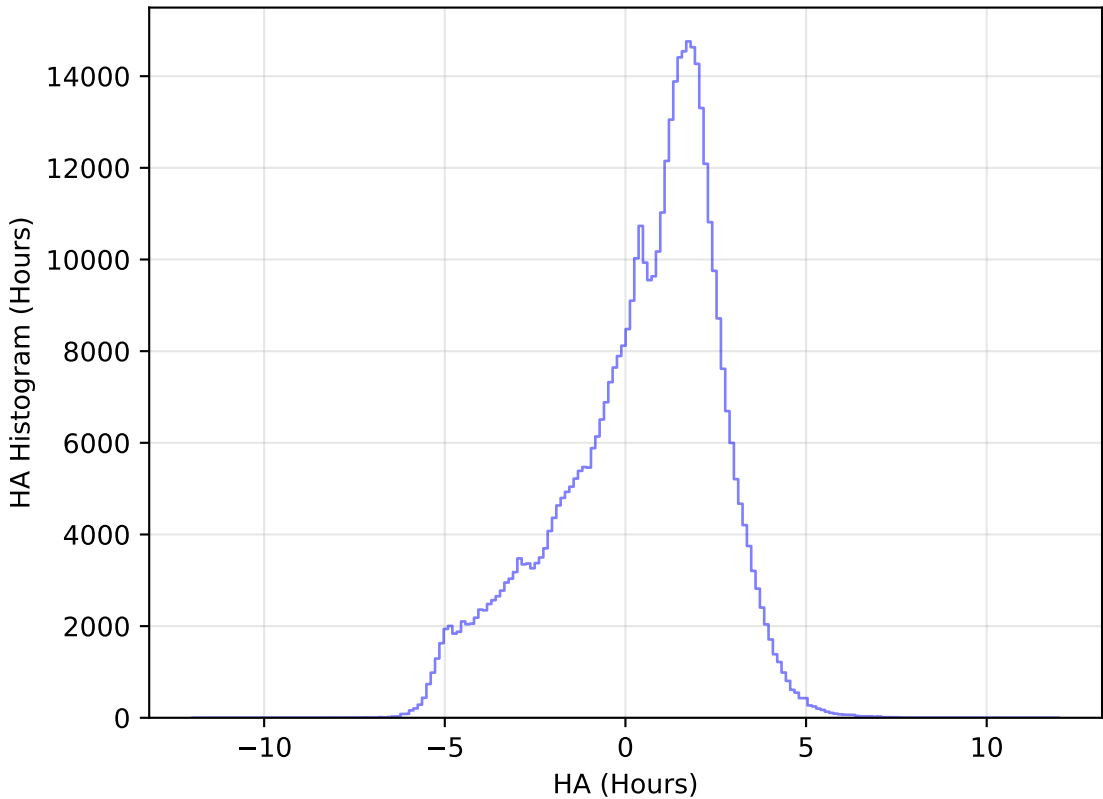
too_elab_r16_d2_griz_v3.4_10yrs All sky r band: HA Histogram
