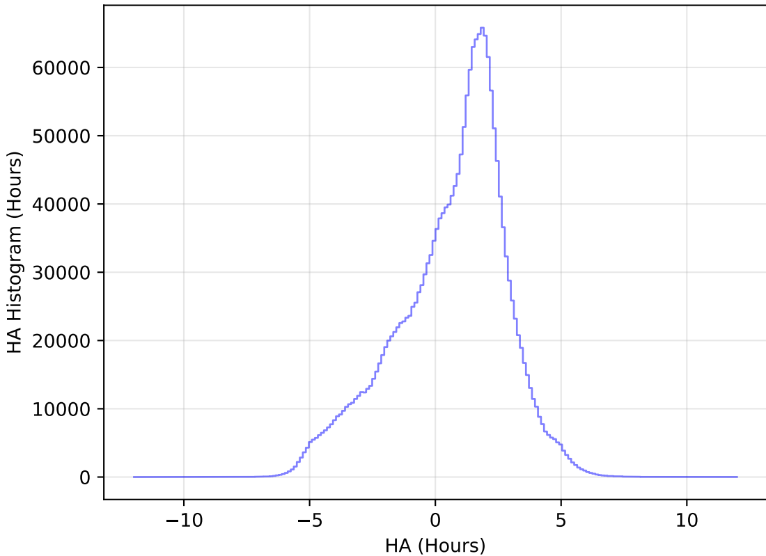
too_elab_r16_d2_griz_v3.4_10yrs All sky all bands: HA Histogram
