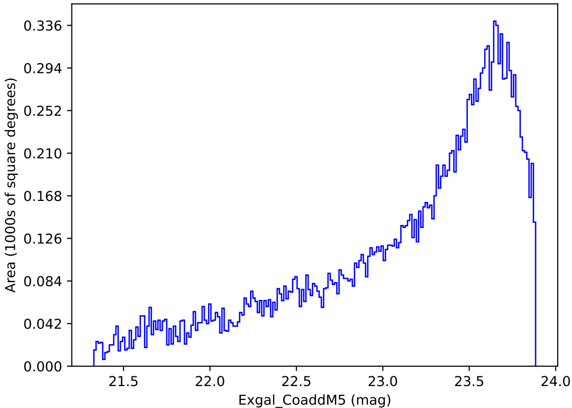
too_elab_r16_d2_griz_v3.4_10yrs Yr 3-4 y band: Exgal_CoaddM5
