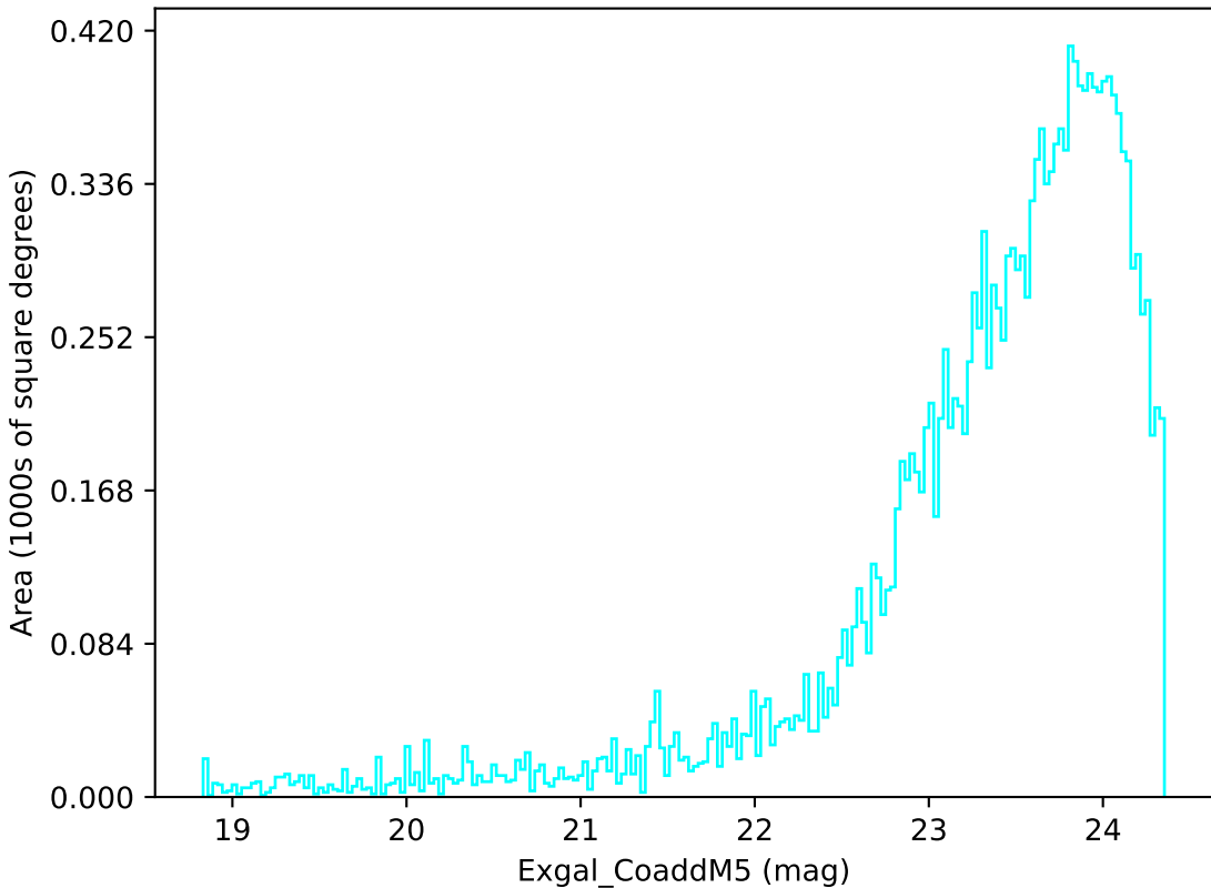
too_elab_r16_d2_griz_v3.4_10yrs Yr 3-4 u band: Exgal_CoaddM5
