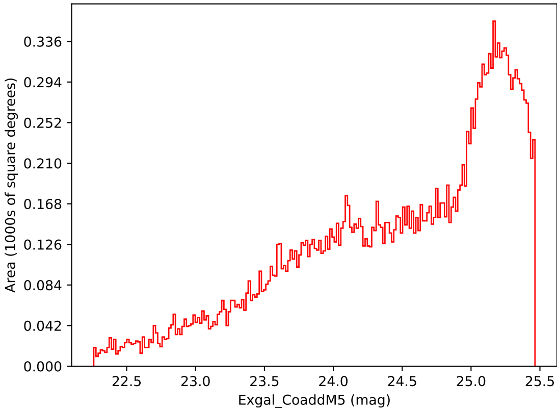
too_elab_r16_d2_griz_v3.4_10yrs Yr 3-4 i band: Exgal_CoaddM5
