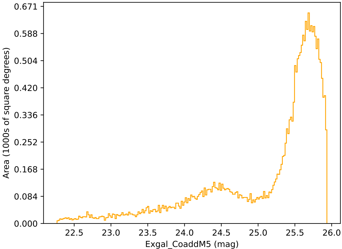
too_elab_r16_d2_griz_v3.4_10yrs Yr 1 r band: Exgal_CoaddM5
