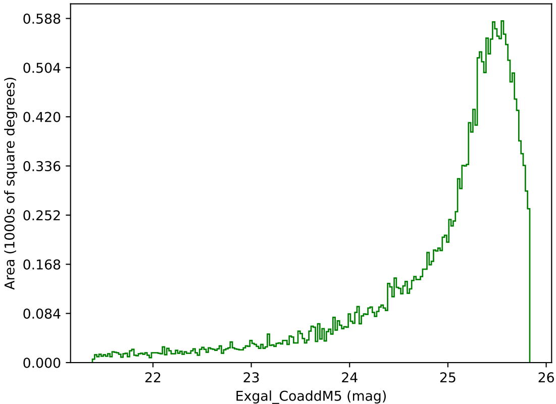
too_elab_r16_d2_griz_v3.4_10yrs Yr 1 g band: Exgal_CoaddM5
