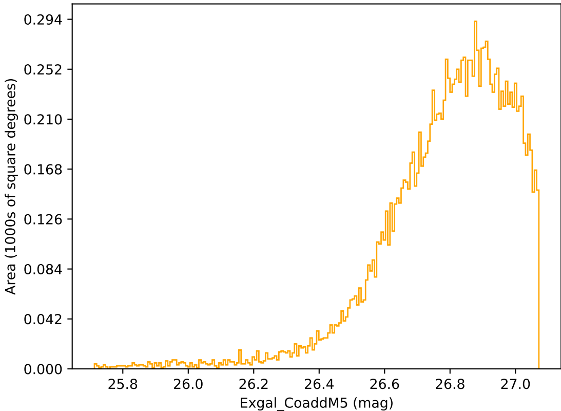
too_elab_r16_d2_griz_v3.4_10yrs WFD r band: Exgal_CoaddM5
