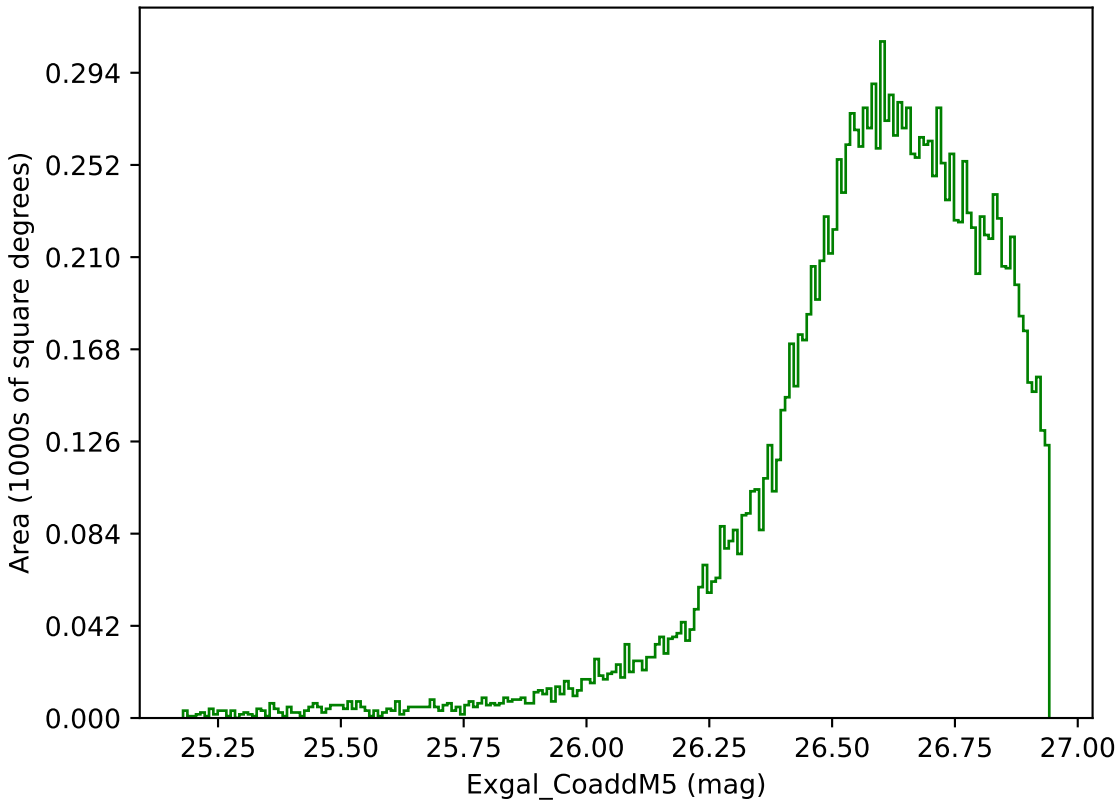
too_elab_r16_d2_griz_v3.4_10yrs WFD g band: Exgal_CoaddM5
